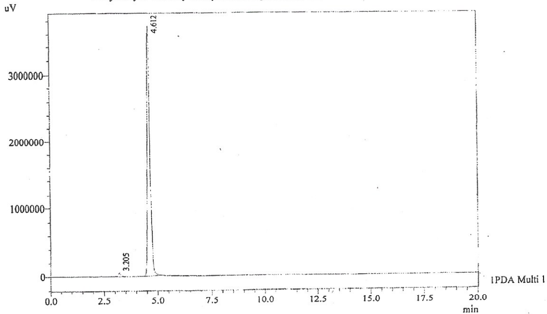
Chromatogram 2'-Hydroxy-5'-methoxy acetophenone D:\promonence\1Data
